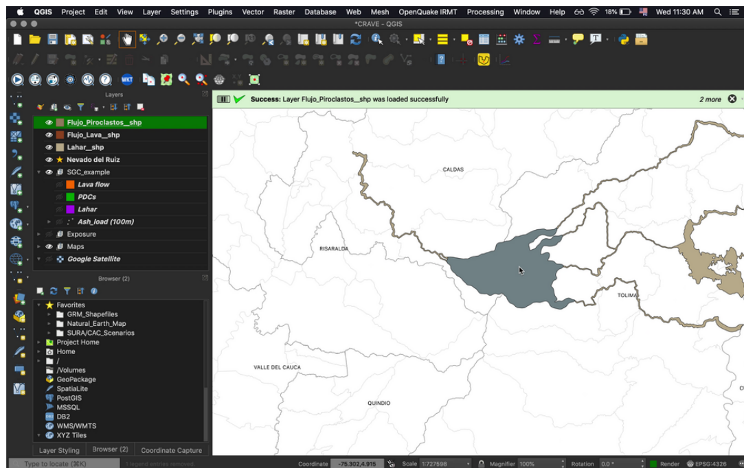
Fig. 17.7: An example of volcano footprint input.
