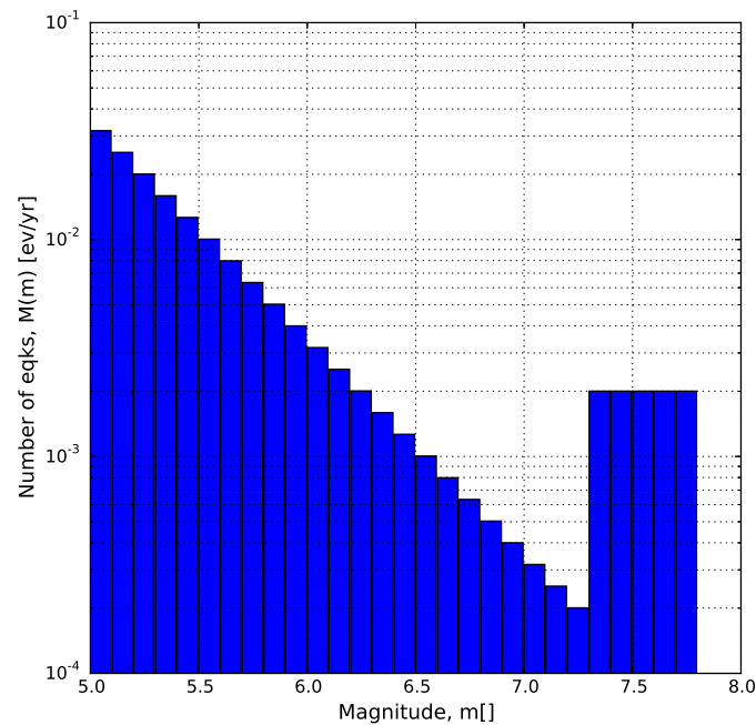
Figure 2.7 – youngs1985 magnitude-frequency distribution.
