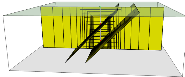
Figure 2.3 – Ruptures produced by the source created using the information in the example .xml file described on page ??.
