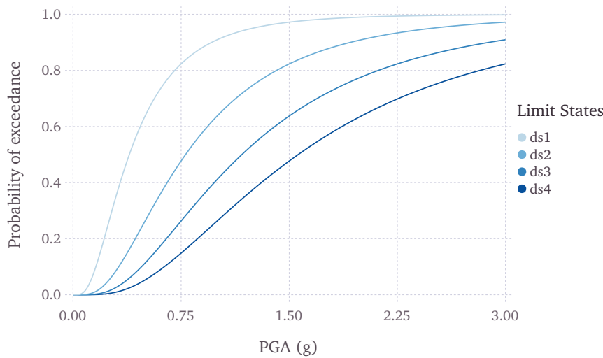
Figure 7.2 – Graphical representation of a continuous fragility model
