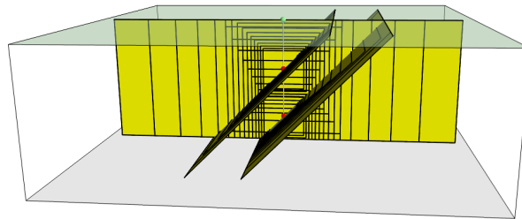
Figure 2.3 – Ruptures produced by the source created using the information in the example .xml file described at page 25.
