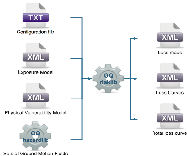
Figure 6.3 – Probabilistic Event-based Risk Calculator input/output structure.
