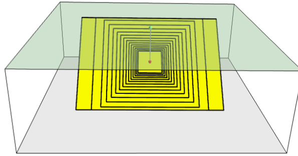
Figure 2.2 – Point source with multiple ruptures. Note the change in the aspect ratio once the rupture width fills the entire seismicogenic layer.
